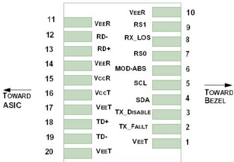
Figure 3, Pin View
